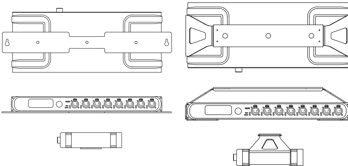
PWACC WMLG Wall-mount Kit
